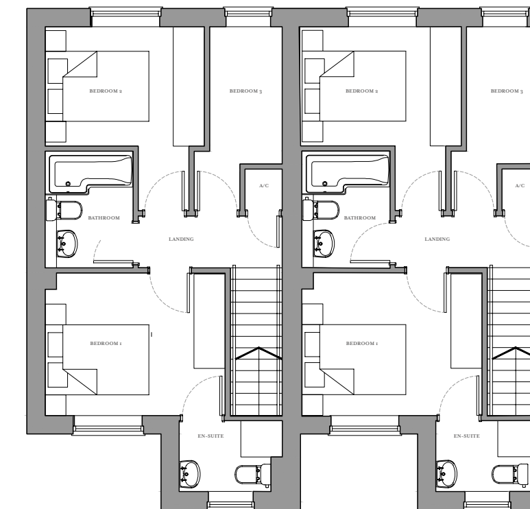
THE MOSELEY FIRST FLOOR
